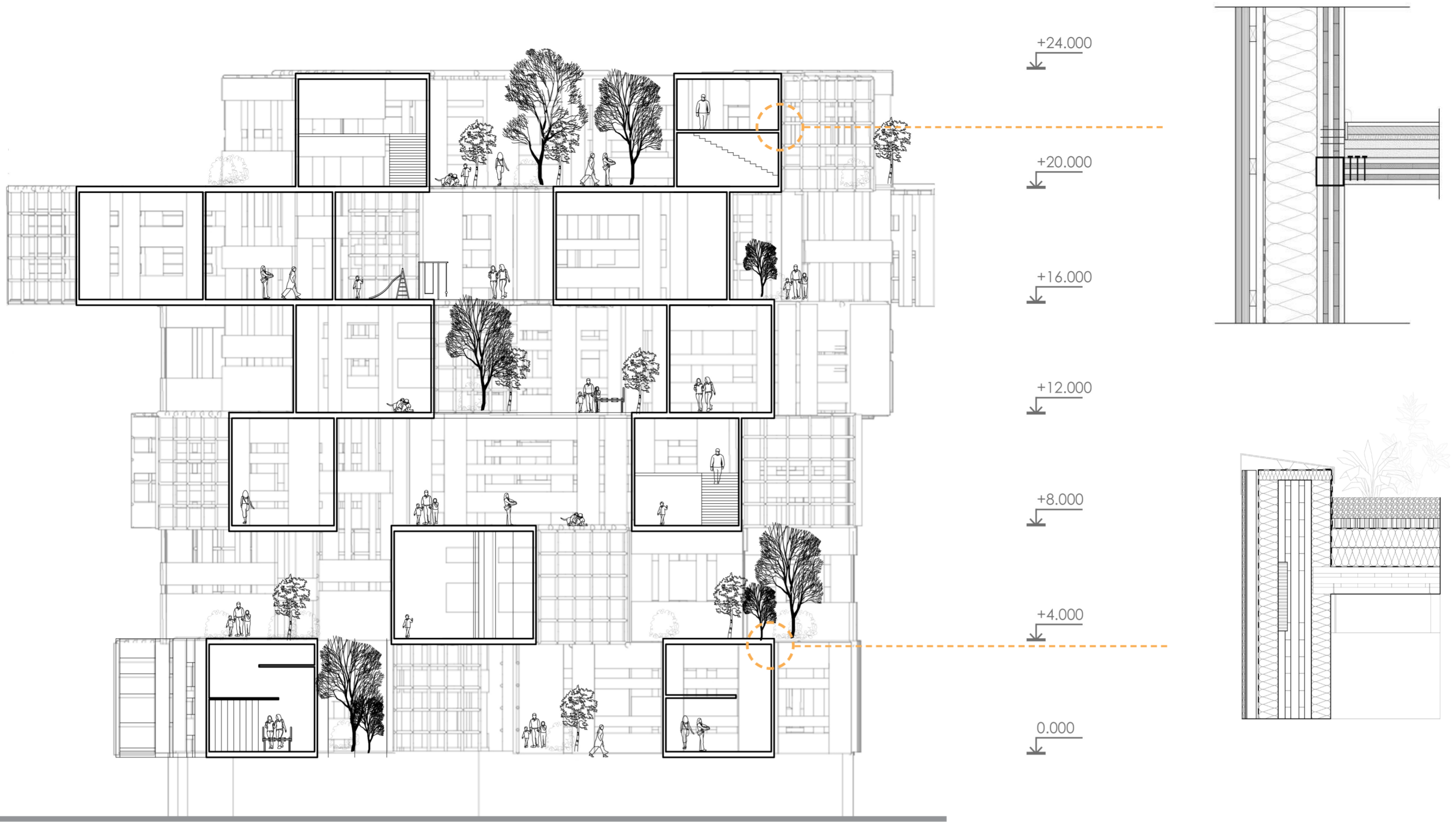
Section
